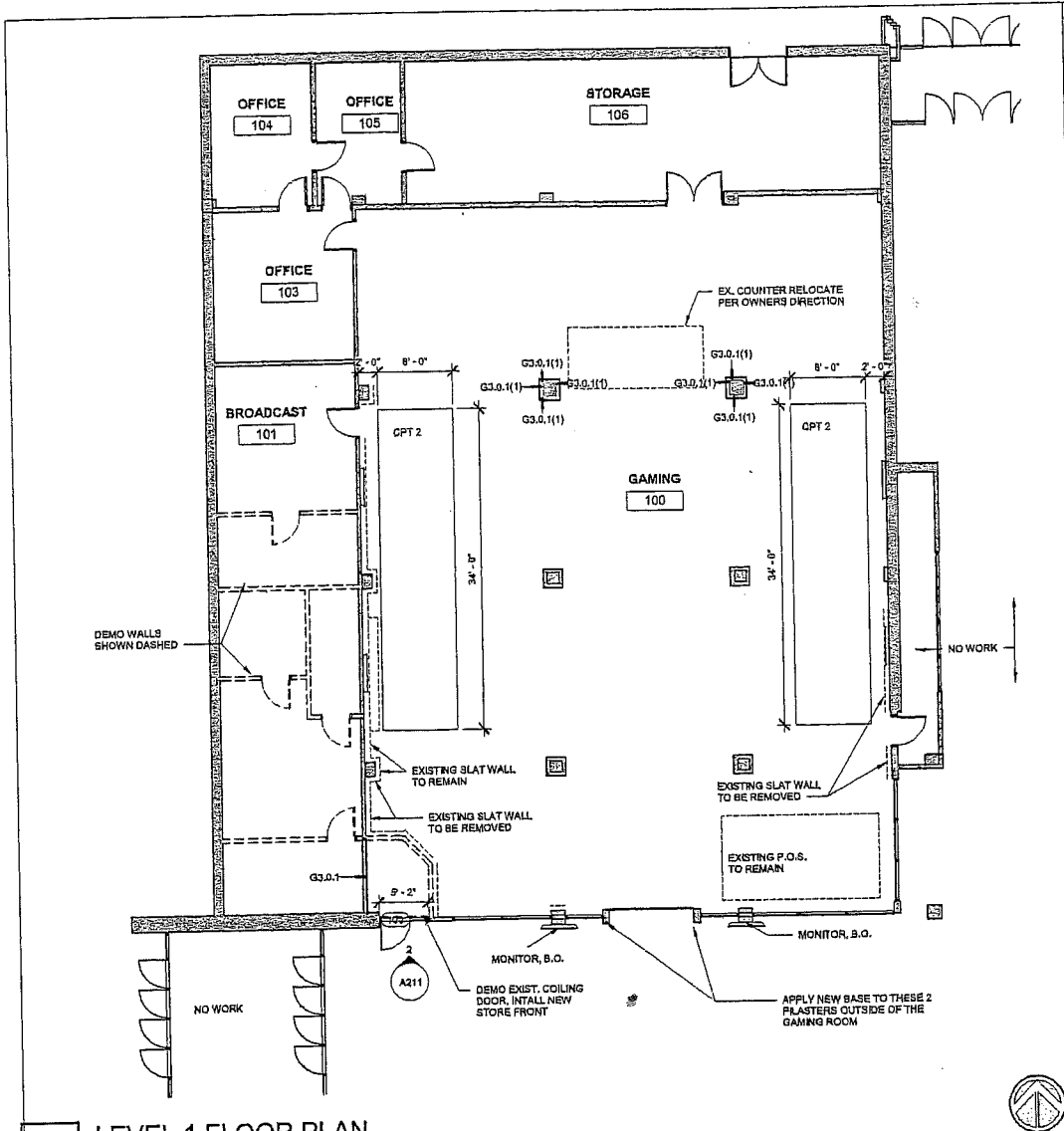
1 LEVEL 1 FLOOR PLAN SCALE: 1/8" = 1'-0"
